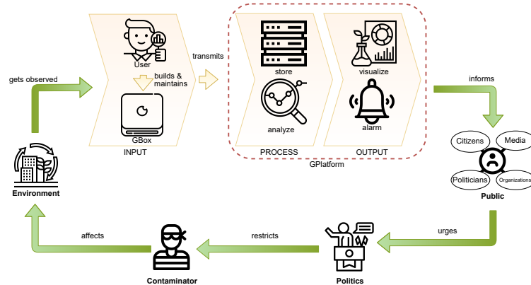
Fig. 1: The control loop behind Guerilla Sensing , taken from Guerilla Sensing [BI21].
